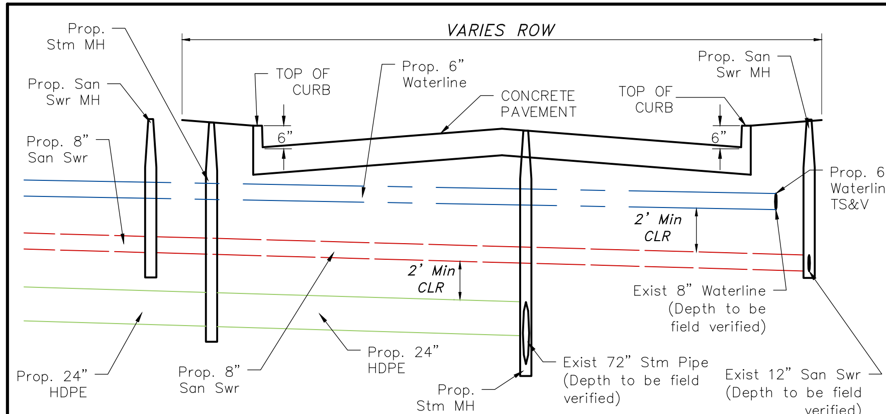
BINGLE ROAD PROFILE VIEW B-B N.T.S.
