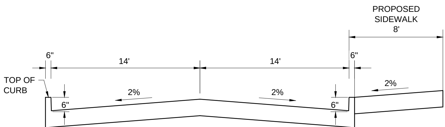
PROPOSED BRIDGE CROSS SECTION A-A N.T.S.
